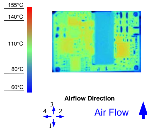
Figure 8. Thermal Image for Airflow Direction 3 (5A output, 70°C ambient, 200 LFM, typical Vin, open frame, unit soldered onto a fixture board)
